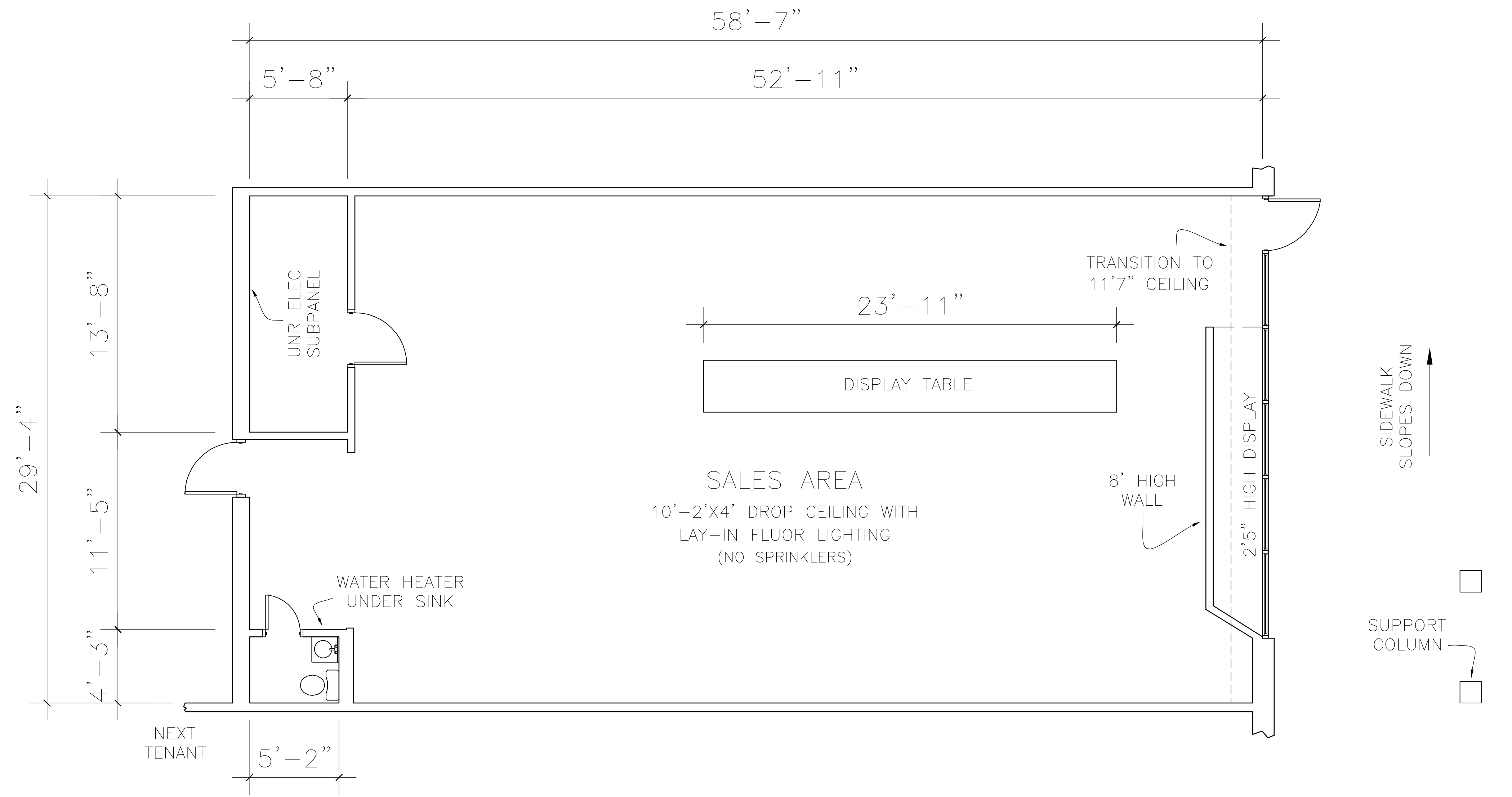
EXISTING FLOOR PLAN: SCALE: 1/4" = 1'
