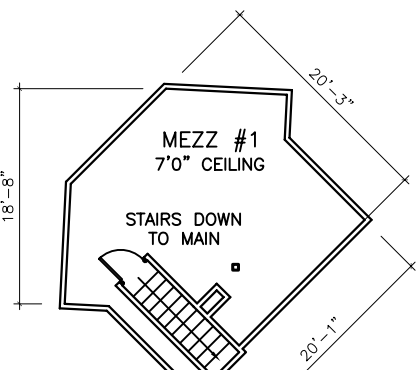
SALES FLOOR MEZZANINE: SCALE: 1/16" = 1'
